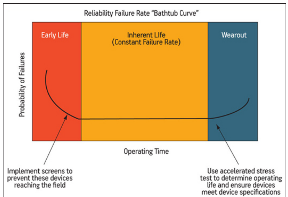
Product reliability “Bathtub Curve”
