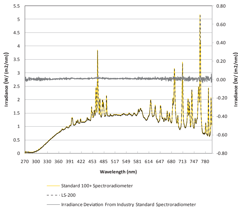
LS-200 vs Common Industry Spectroradiometer
