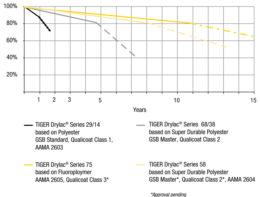
Figure 6: Comparison of Florida weathering results of various exterior grade powder coatings
