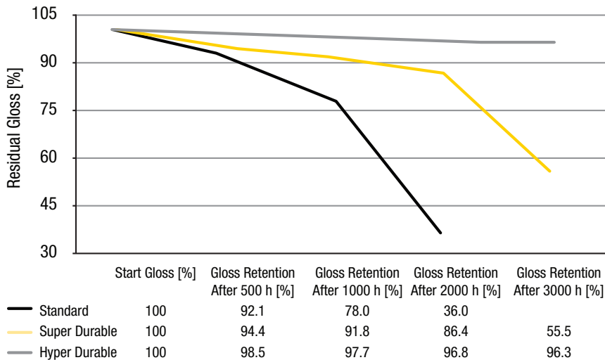
Figure 7: Comparison of xenon weathering results of various exterior grade powder coatings and correlation to natural Florida weathering. Accelerated testing was performed in an Atlas Ci4000 Weather-Ometer®, and natural weathering was performed at Atlas' South Florida Testing Services.
